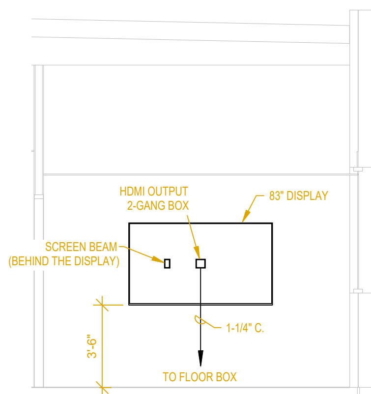
6 CONFERENCE B107 AND E128 SCALE: 1/4" = 1'-0"
