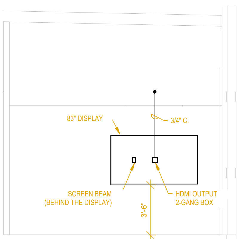
4 DIRECTOR B106 AND OFFICES SCALE: 1/4" = 1'-0"
