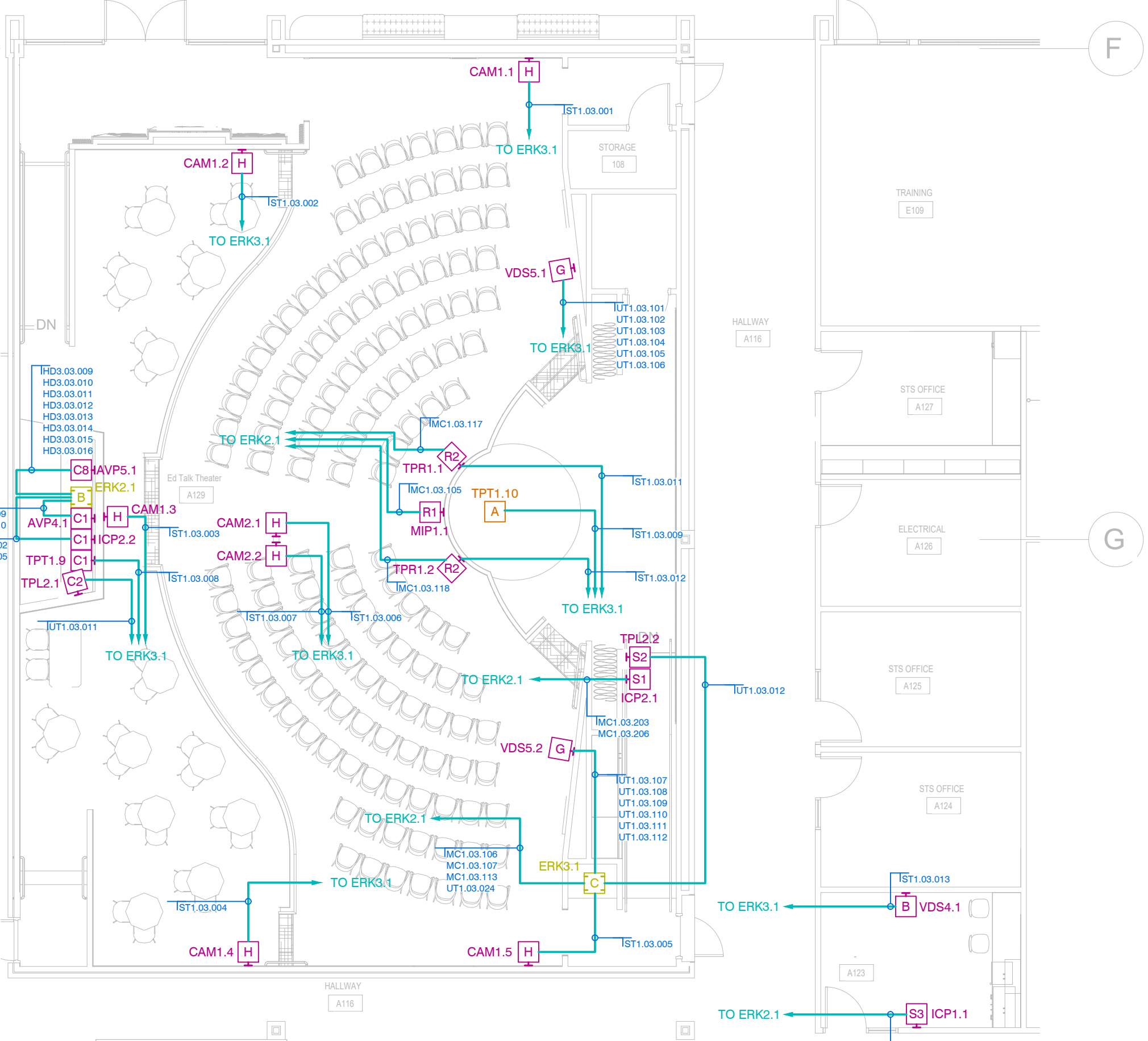
2 AUDIOVISUAL SYSTEM - ED TALK THEATER FLOOR AND REFLECTED CEILING PLANS SCALE: 1/8" = 1'-0"
