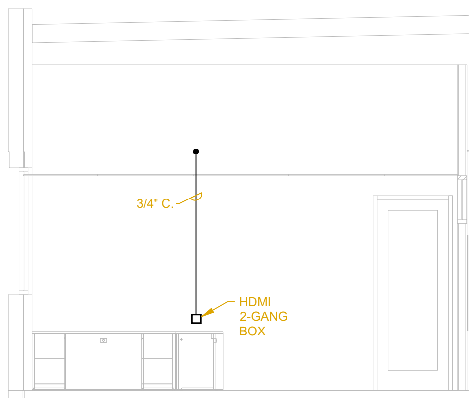
5 DIRECTOR B106 AND OFFICES SCALE: 1/4" = 1'-0"
